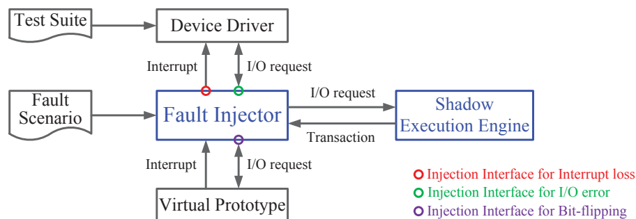
Figure 5.11: Fault Injection Framework Using Runtime Shadow Execution
