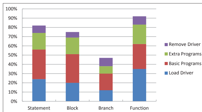
Figure 4.6: Code Coverage Results for E1000
